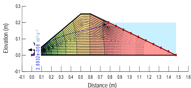
Fig. 1. Numerical analyses by GeoStudio software for soil 1 and upstream slope 1:3.5: a) seepage, b) factor of safety; source: own study
